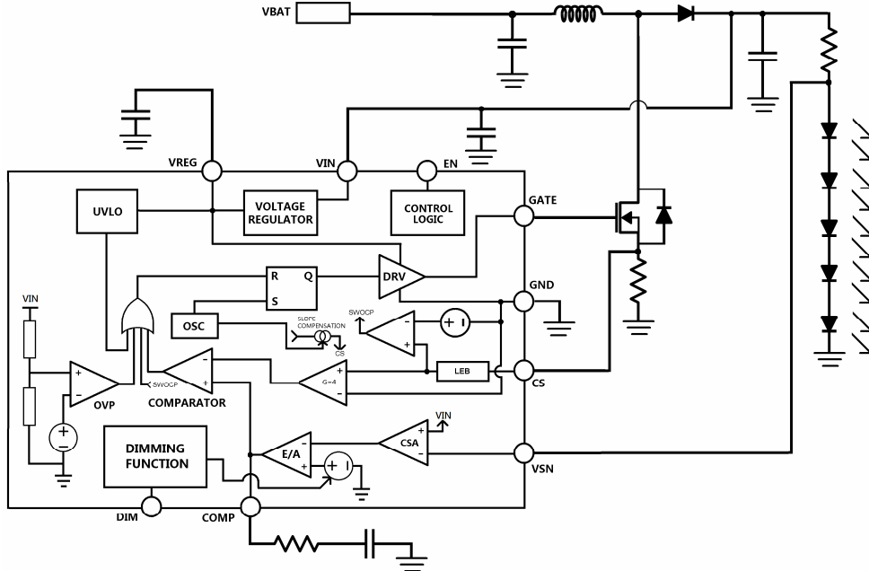
Boost Converter which is for V_{BAT} < V_{LED} .
